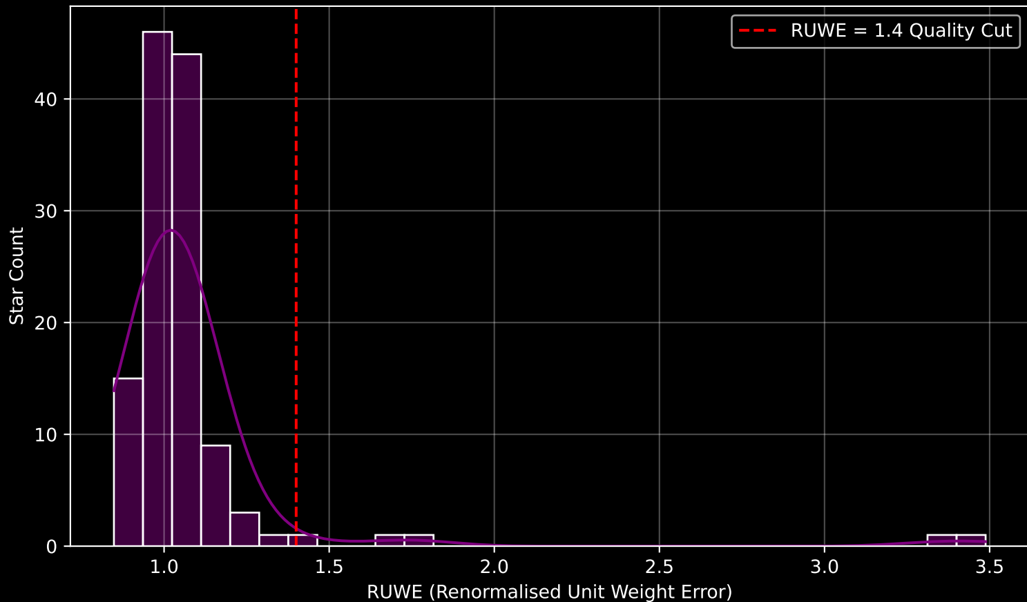
GAPOGEE DR17 Field [033+00] RUWE Distribution (n= 123)
