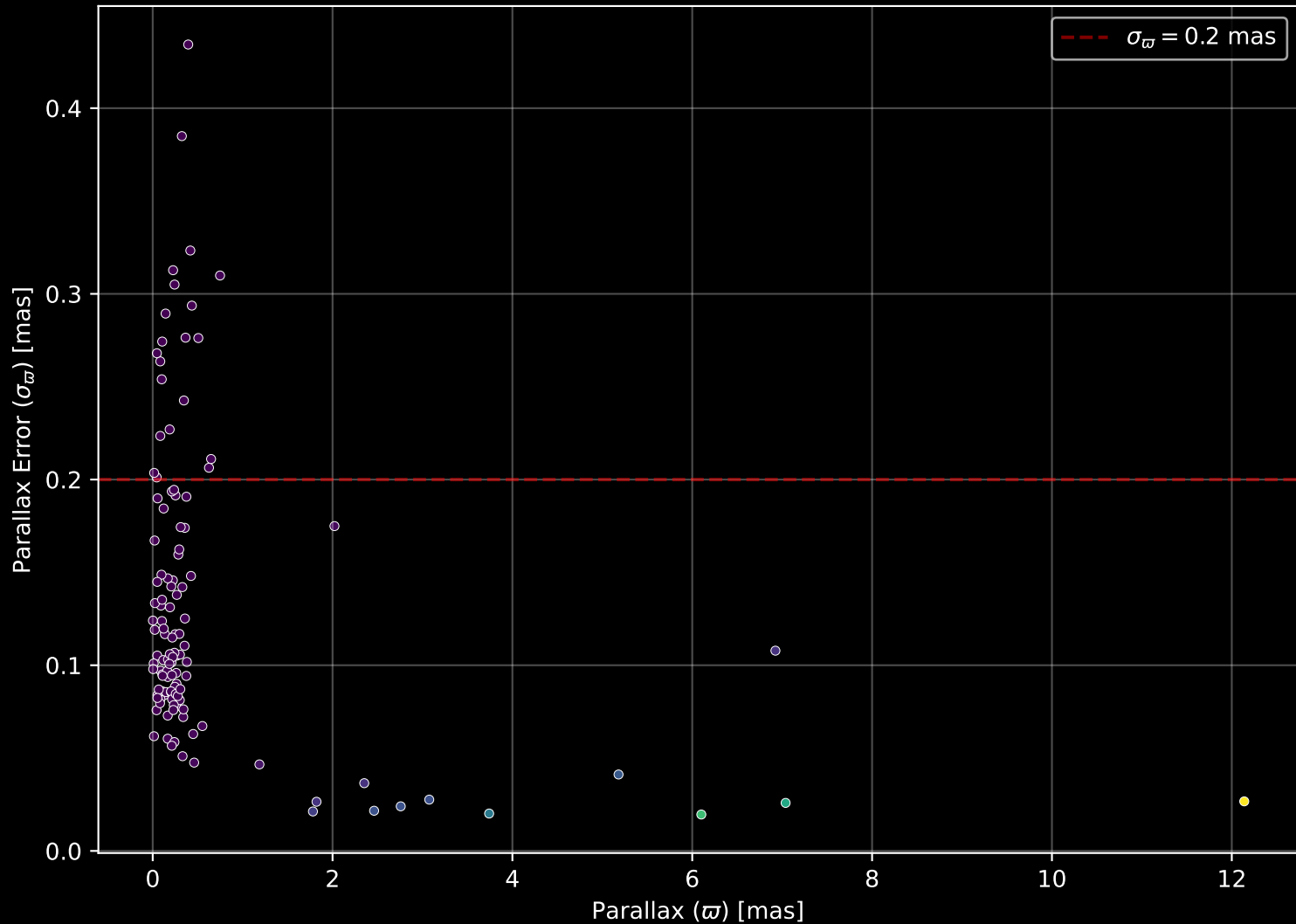
APOGEE DR17 Field: [033+00] Parallax Quality (n= 123)
