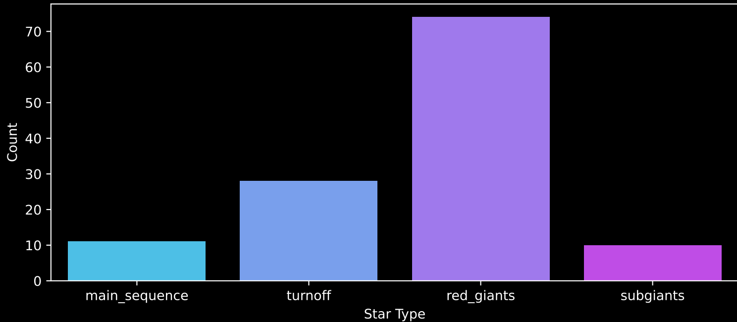
APOGEE DR17 Field: [033+00] Count plot of Star Type
