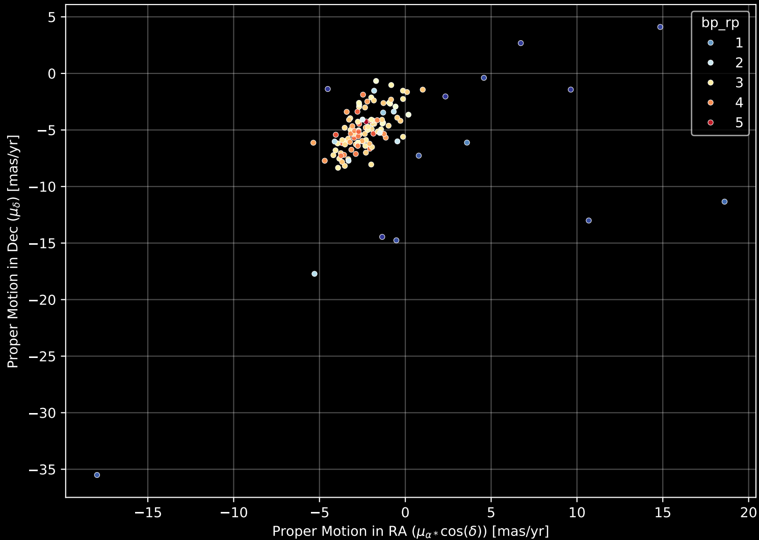
APOGEE DR17 Field: [033+00] Proper Motion Diagram (n= 123)
