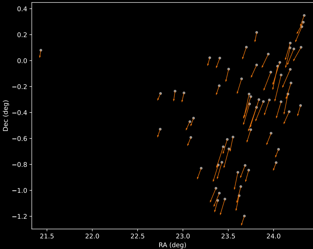
APOGEE DR17 Cluster 2 Proper Motion Vectors (n=62)
