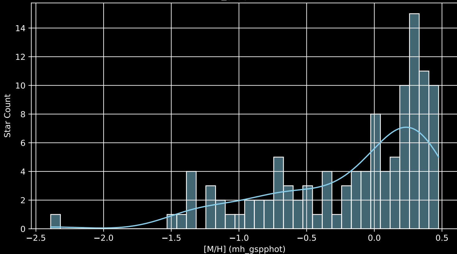
APOGEE DR17 Field: [033+00 [M/H] (mh_gspphot) (n= 113)
